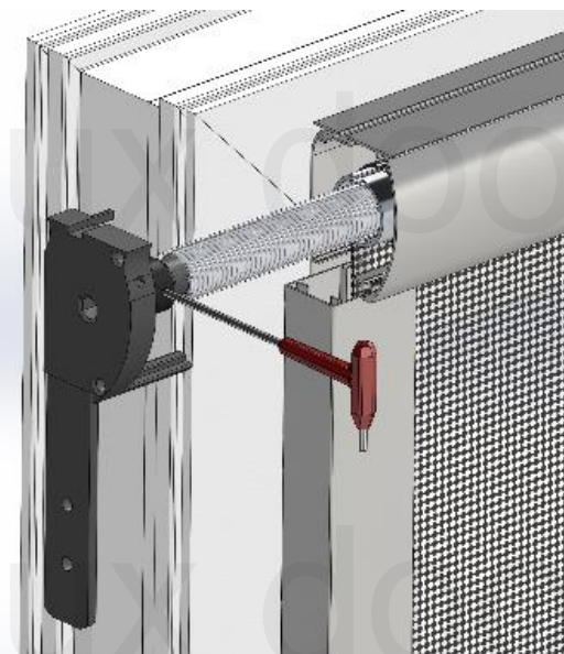
Regulator opruge.
