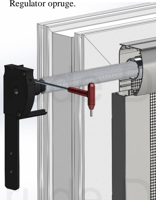
Regulator opruge.
